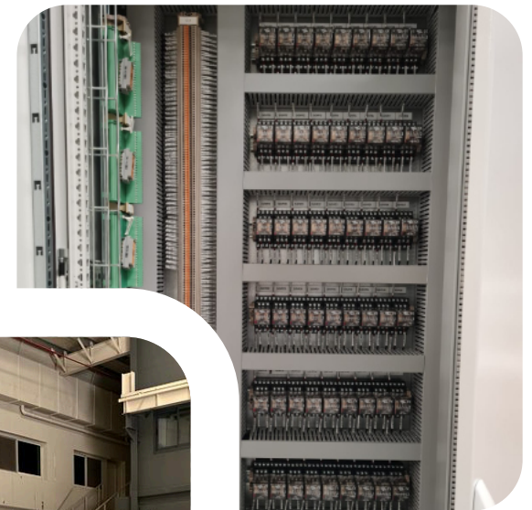
Relay Panel
